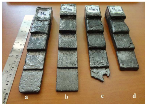
Fig. 5. Casting sample of nodular cast iron produced with different coating thickness variation of (a) 0 (without coating), (b) 200 \mu\text{m} , (c) 500 \mu\text{m} and (d) 1300 \mu\text{m}
